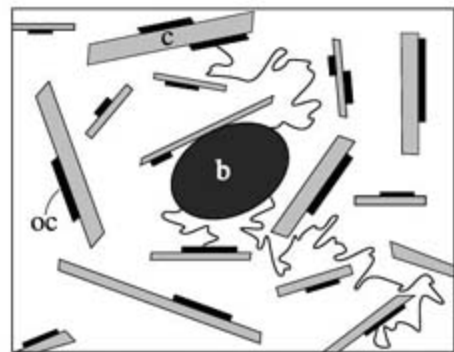
Fig. 1. Schematic illustration of the main features of our model. In a porous medium characterized by its porosity \phi , organic carbon (oc) is associated with the surface area of clay (c) and other minerals. Extracellular enzymes are emitted from randomly distributed bacteria (b), diffuse through the medium, and hydrolyze organic matter upon contact. For simplicity, diffusive paths show only first encounters of enzymes with solid surfaces; later encounters occur until enzymes become inactive, at a specified rate \alpha . Except for the random distribution of bacteria, each of these features is contained in a more detailed model proposed by Vetter et al. (21).
